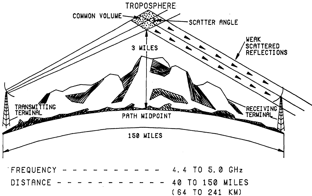
Figure 1-1 Tropospheric scatter radio system.
