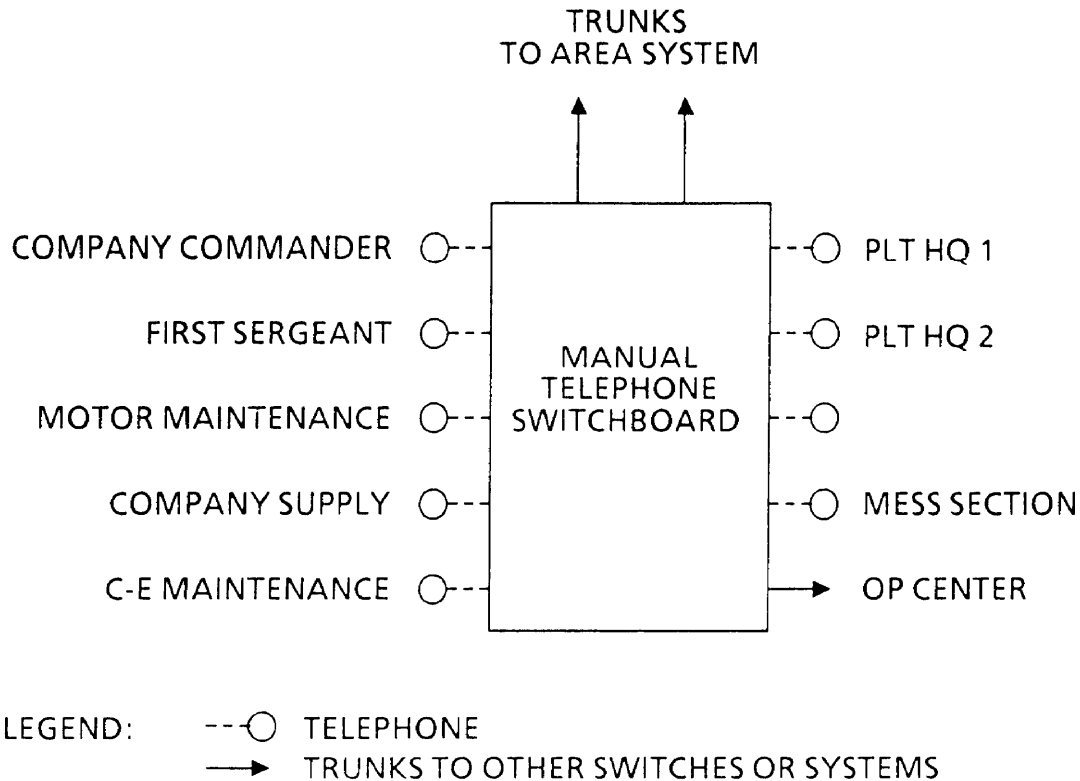
Figure 6-2. Signal Troopscatter Company (Heavy) Type Telephone Net.
